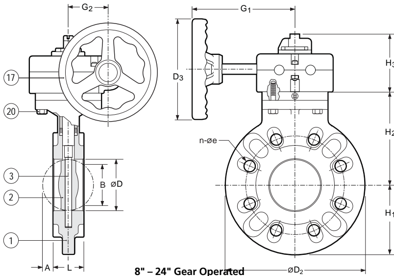
8" – 24" Gear Operated
